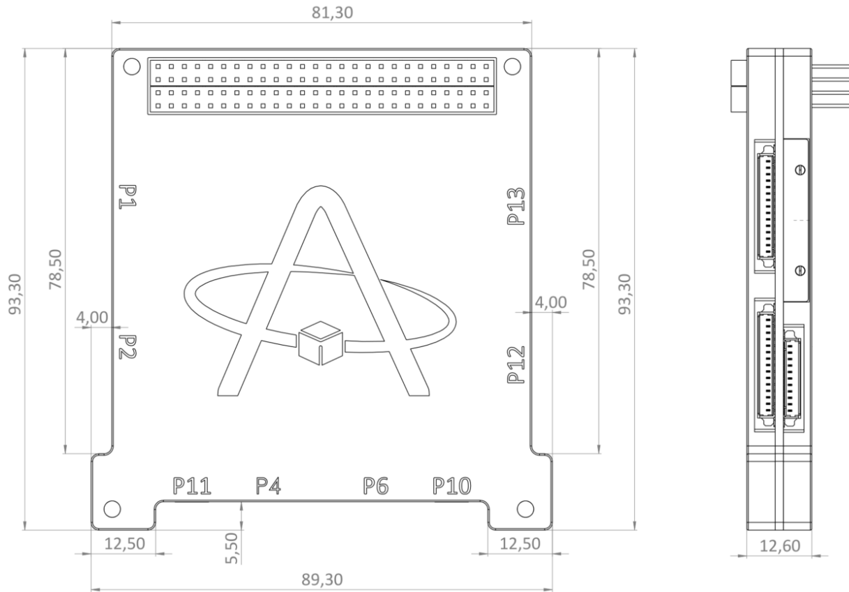
Figure 3 : Mechanical drawings
